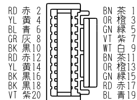
VIEW A-A'
