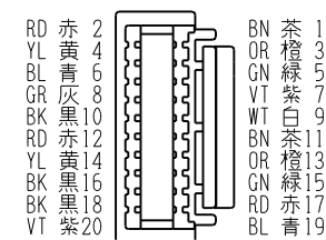
VIEW A-A'
