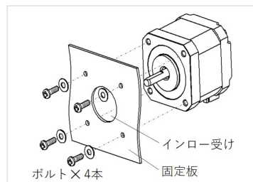
PMSB-B28 PMSA/C-B42
